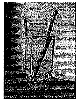
A demonstration of refraction.
